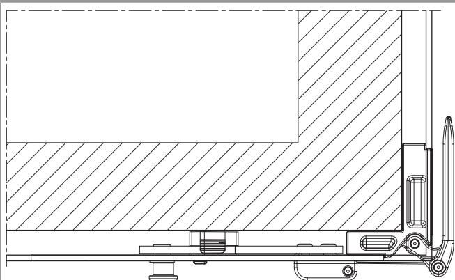
Sash in close position
