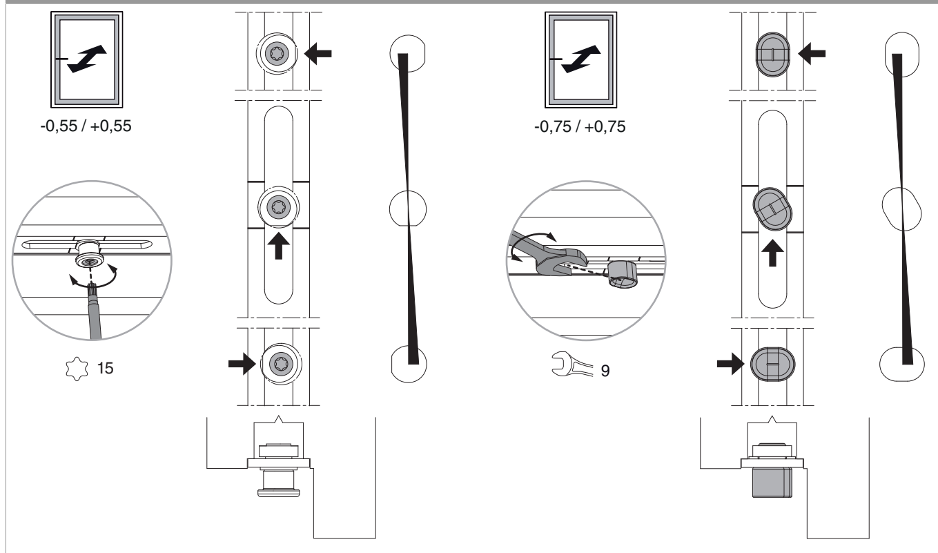
i.S. locking cams and standard locking cams
