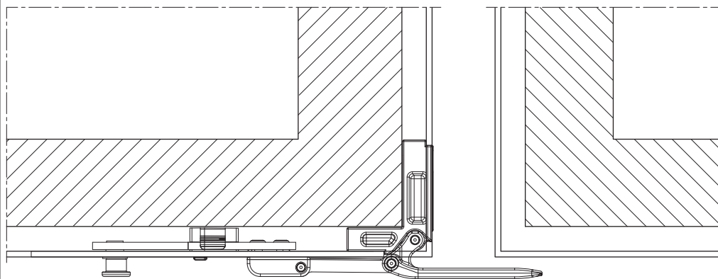
Sash in close position
